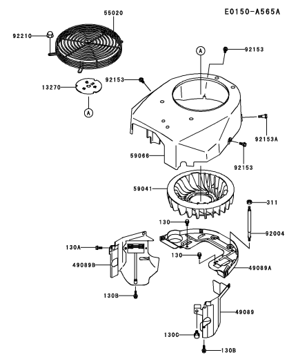
B-07 COOLING-EQUIPMENT
