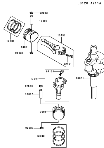
B-04 PISTON/CRANKSHAFT
