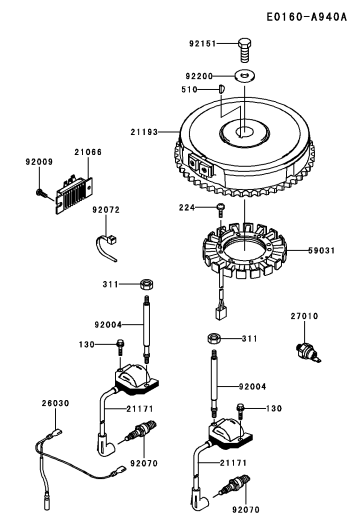
B-08 ELECTRIC-EQUIPMENT
