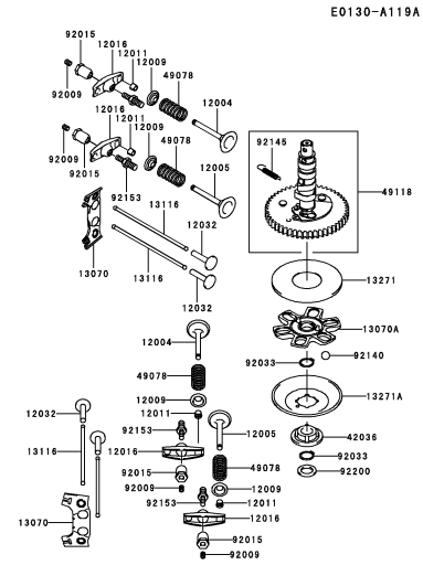
B-05 VALVE/CAMSHAFT
